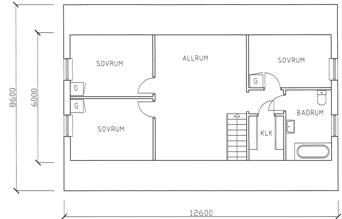
PLAN 2
