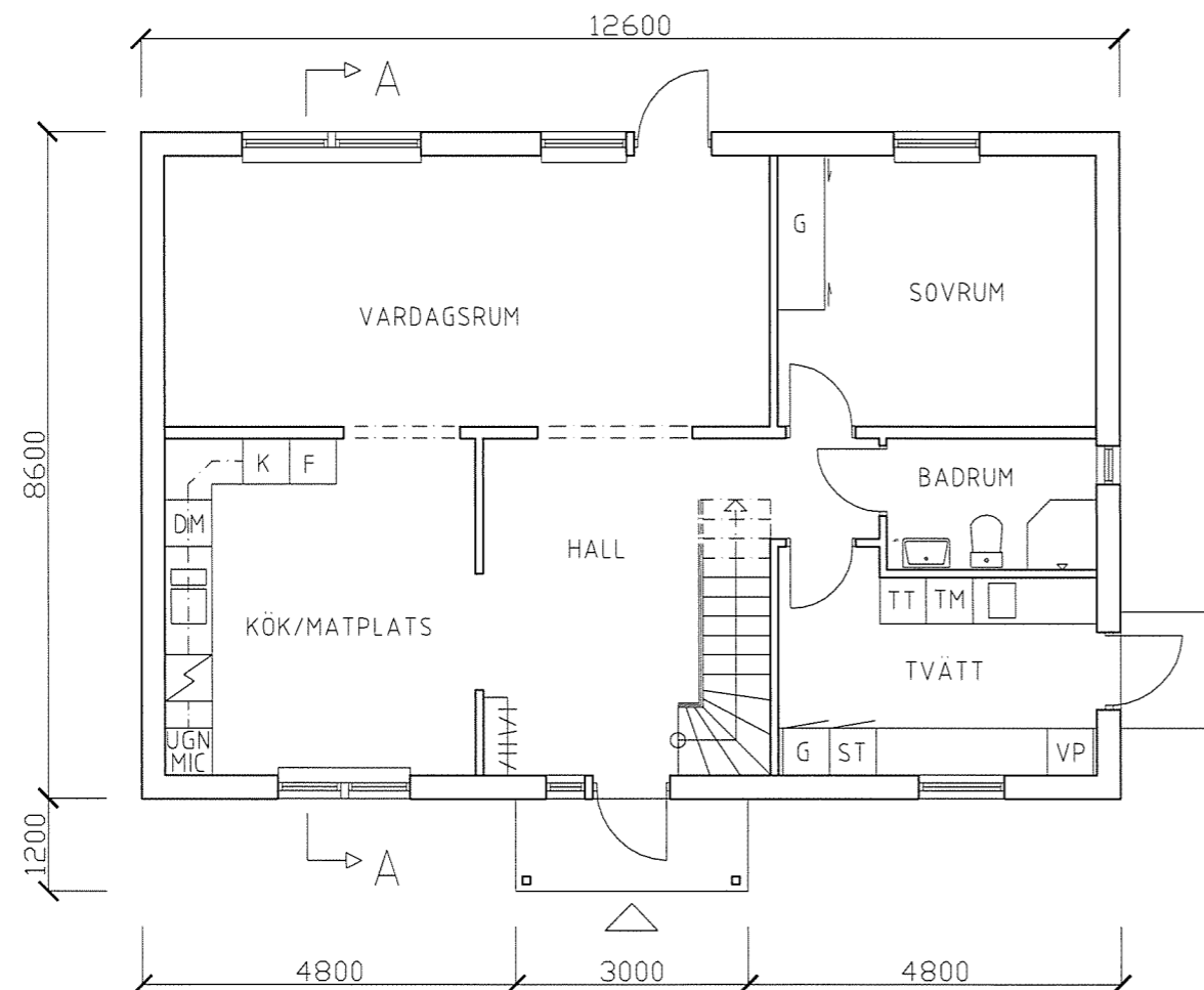
PLAN 1
