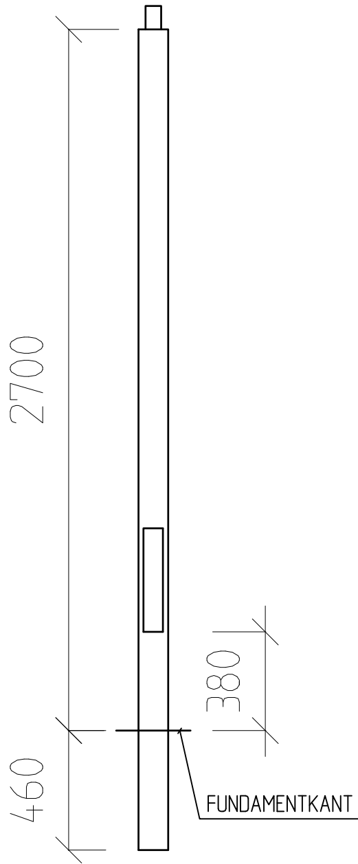
STOLPE POS L2
