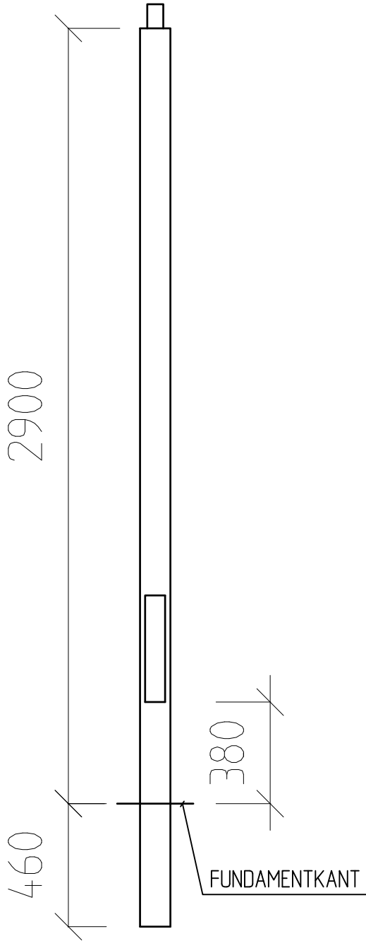
STOLPE POS L1, L3
